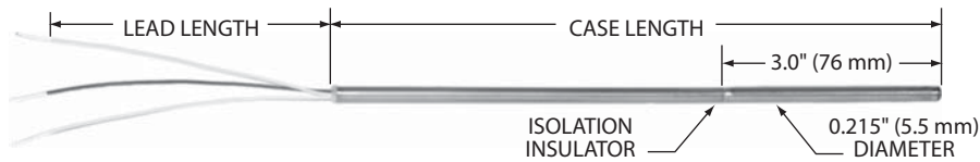
RTD STAINLESS PROBE
