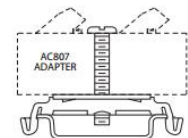
AC807 adapter for EN50022
